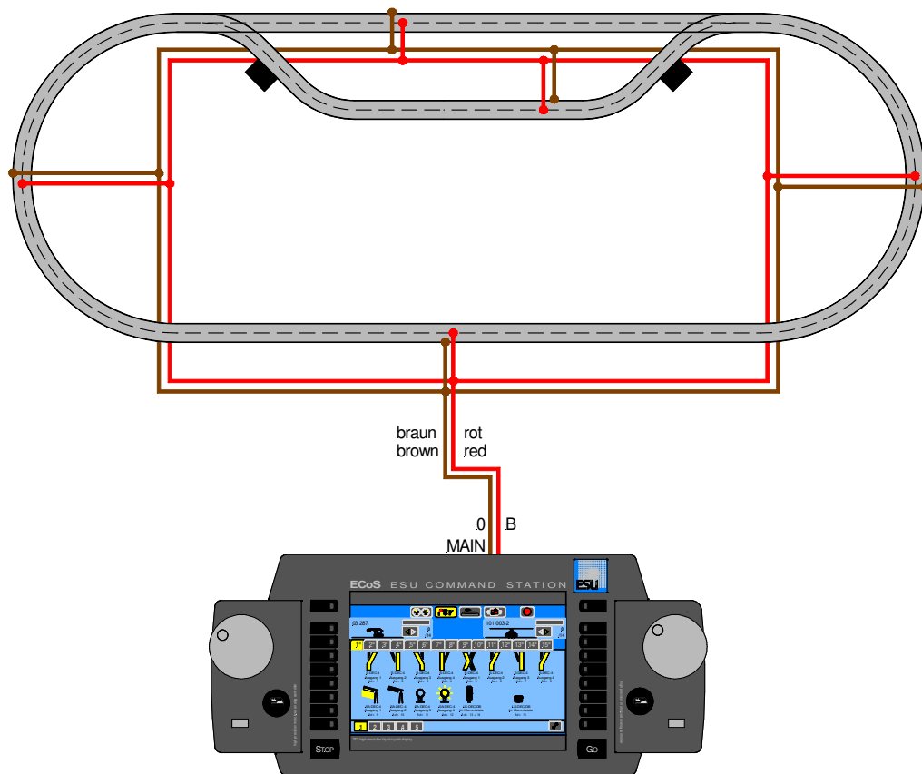
■ Connection of the ECoS Digital Central Unit (page_1053)
