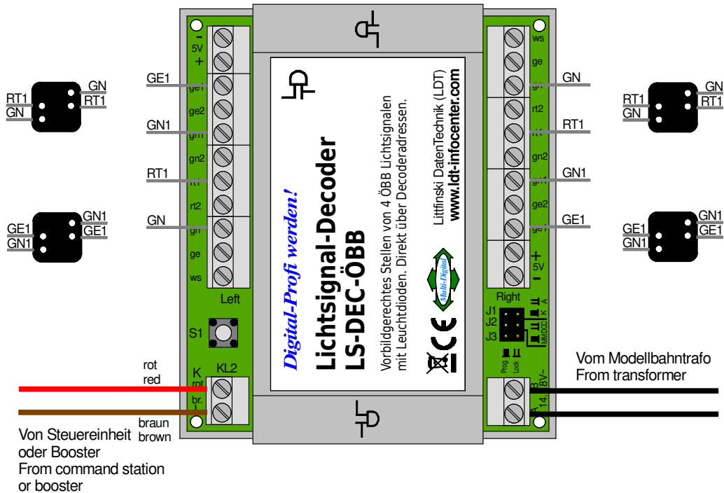
■ Sample Connection of Shunting- and Dwarf Signals (page_270)
