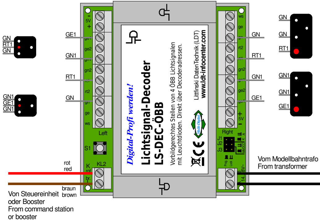
Sample Connection of Safety Signals (page_269)
